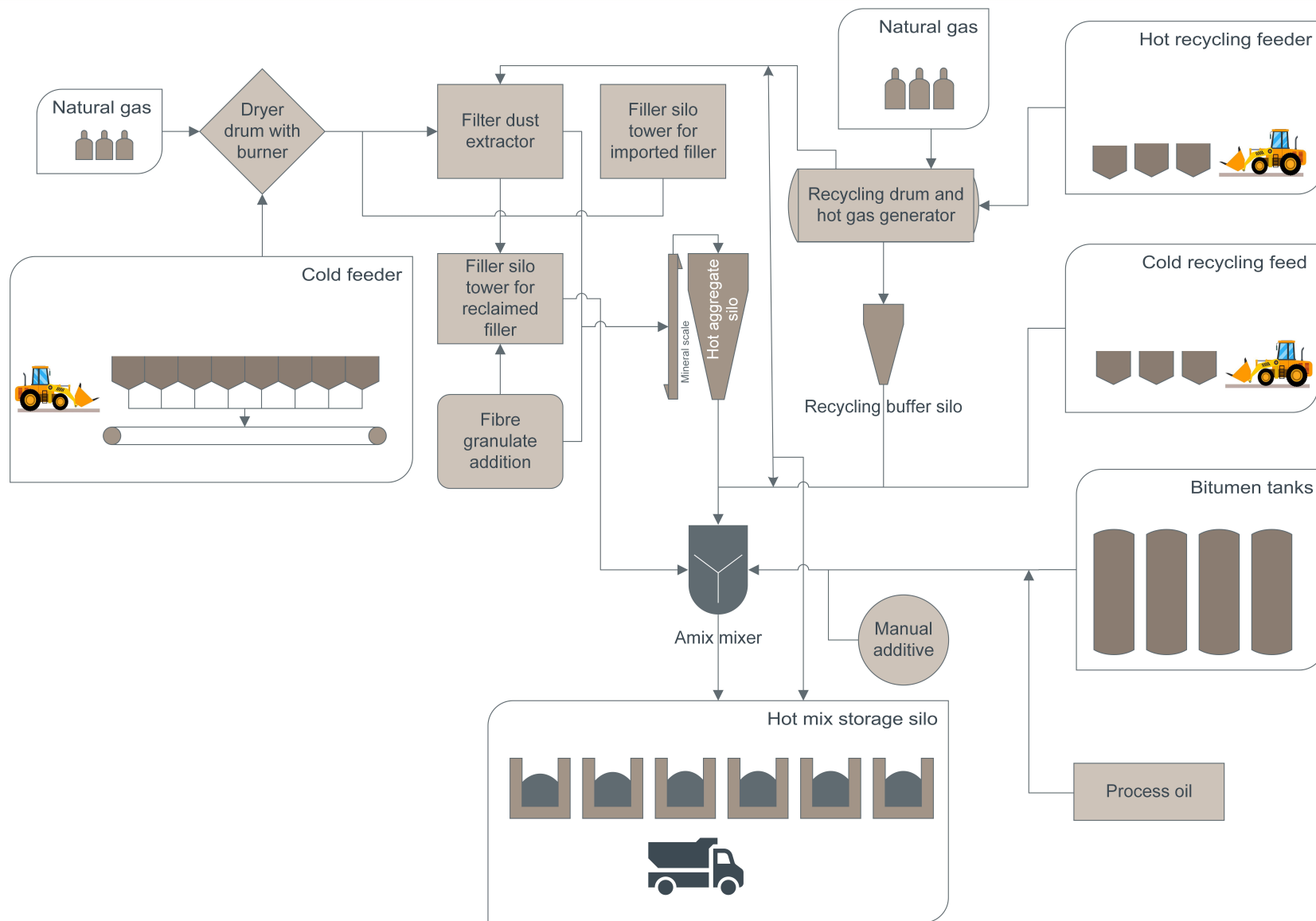
Figure 3.14 Asphalt production process diagram
