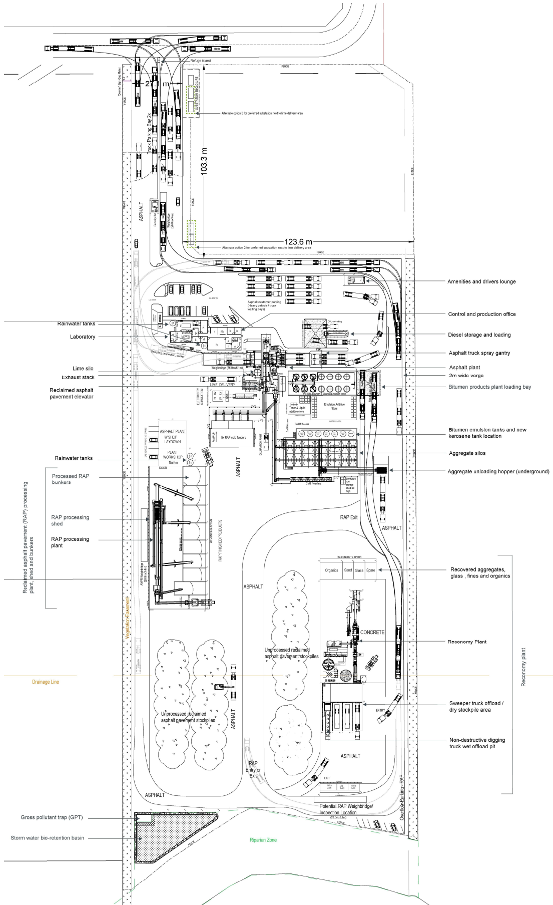
Figure 4 Site Layout
