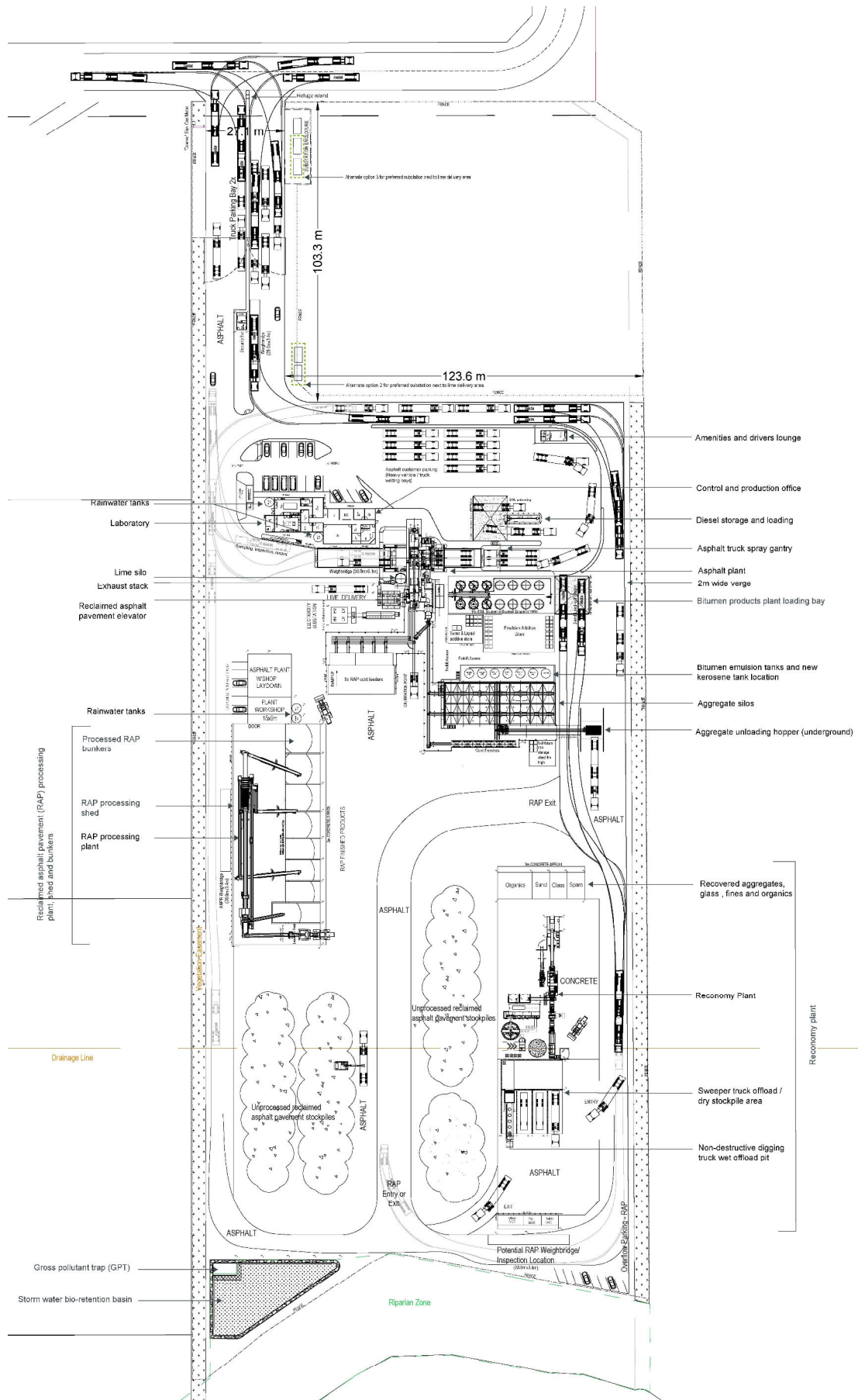
Figure 4 Site Layout
